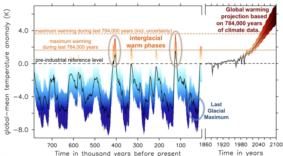
Fig. 1. Global mean temperature anomaly with respect to preindustrial reference level. Left panel: Reconstruction of last 784,000 yrs. Right panel: Global warming projection to 2100 based on newly calculated paleoclimate sensitivity.
