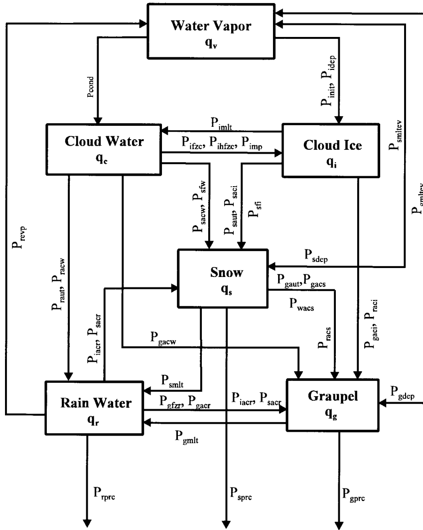
FIG. 3. The cloud microphysical processes considered in the model. See appendix B and Table 1 for an explanation.
